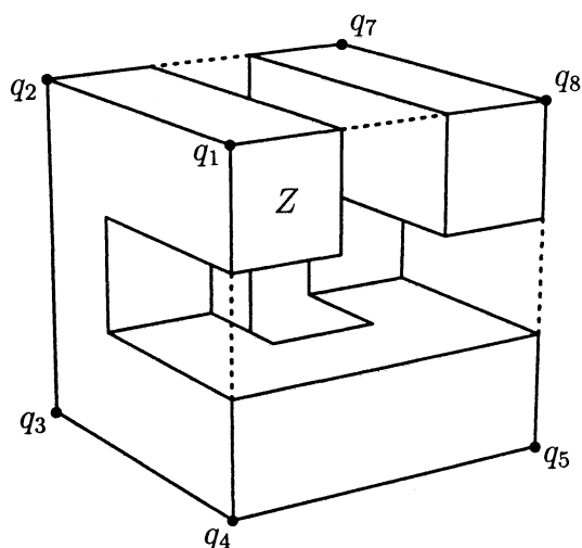
The proof of 3.2.
