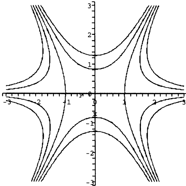
Figure 1. — Phase portrait, n = 4
