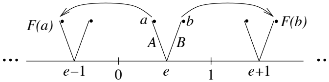
Figure 1.4. The set \text{Rot}(F) = \{-1, 0, 1\} is not connected and is not equal to \text{Rot}_{\mathbb{R}}(F) = \{0\} .
