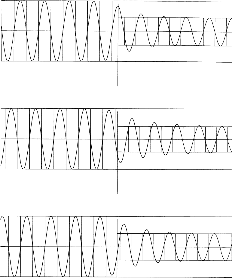
FIG. 1. — Three stationary solutions for the non-homogeneous equation. The parameters are a_R = 0.5 , a_L = 1.0 , \varepsilon = 0.7 , c_L = 0.577,35 . The other parameters are adapted to make a smooth solution.
