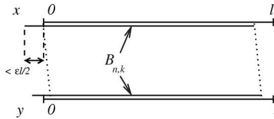
Fig. 4. Coupling of large \mathcal{P} -names.
