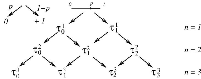
Fig. 3. Representing k_n(x) as the sum of n independent Bernoulli random variables.
