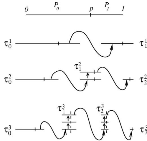
Fig. 1. Cutting and stacking construction of the Pascal adic transformation.
