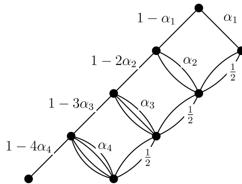
Fig. 5. The invariant measures when T is restricted to the paths x with vertices (n, k_n(x)) with k_n(x) = 0 or 1 for all n .
