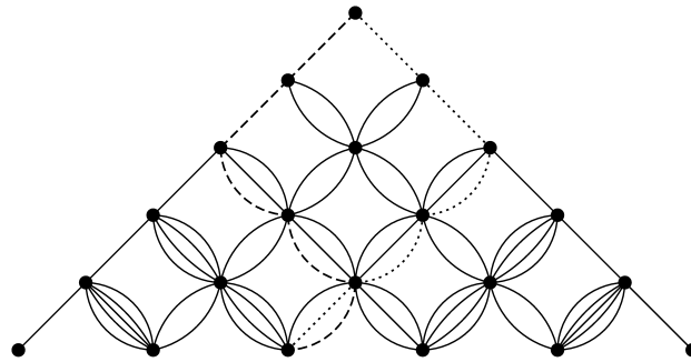
Fig. 2. The dotted path maps to the dashed path.
