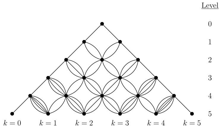
Fig. 1. The Euler graph down to level 5.
