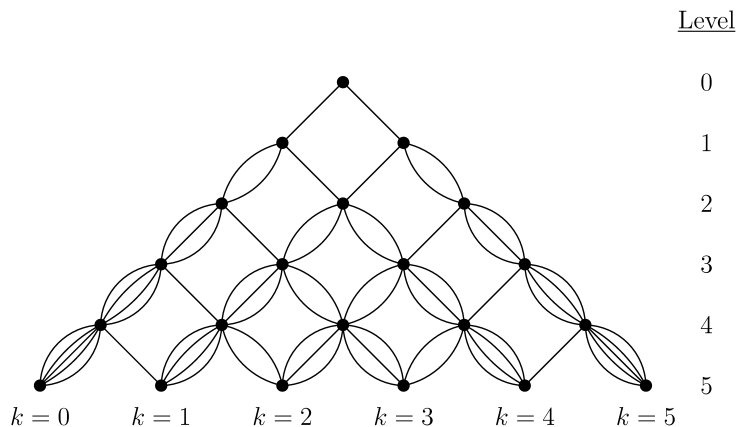
Fig. 6. The reverse Euler graph.
