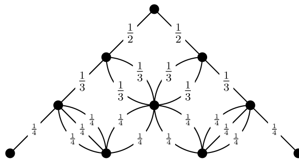
Fig. 3. The symmetric measure given by weights on edges.
