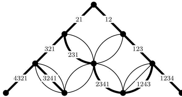
Fig. 4. Some cylinders and their corresponding permutations.
