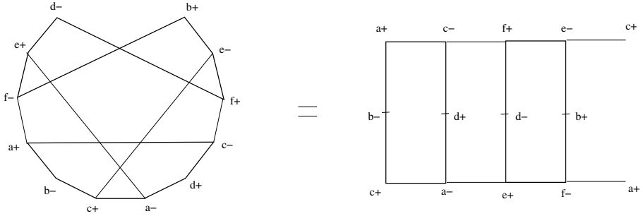
FIGURE 1. The link L and its labelling
