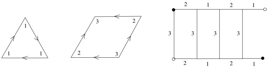
FIGURE 2. Description of the complex X
