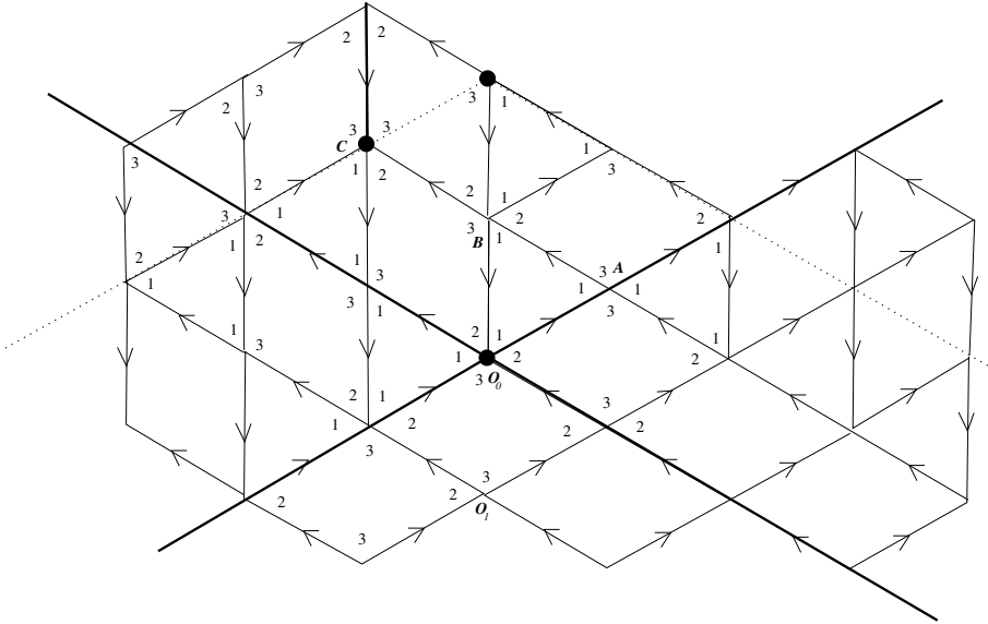
FIGURE 4. Exponential mesoscopic rank of the complex X
