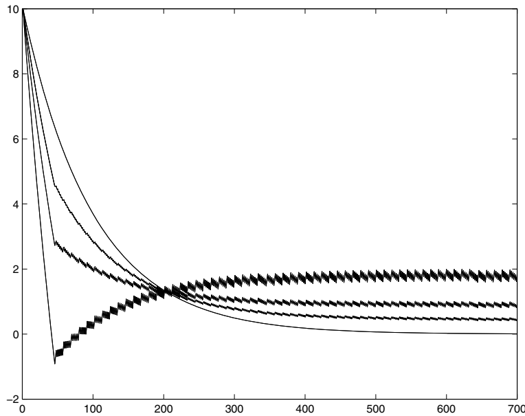
FIGURE 3. State trajectory for the system of Figure 2. Chattering around the hyperplane \mathcal{H} is due to the discontinuous behavior of \omega that jumps between \bar{\omega} and -\bar{\omega} .
