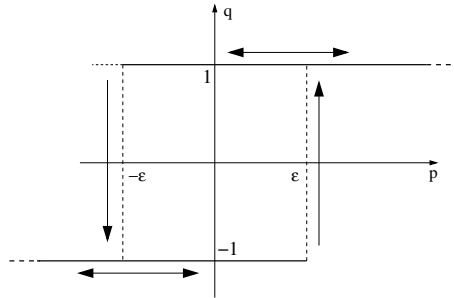
FIGURE 7. Delayed thermostat with thresholds \pm\varepsilon .
