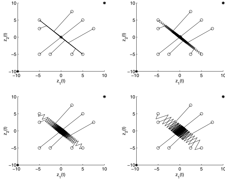
FIGURE 5. State trajectory in the phase plane from different initial states (circles). In evidence the two equilibria \pm \frac{D\bar{\omega}}{k} = \pm [10 \ 10]' (star). (Top left) g_3 as in (2.3) and C_2 > 0 ; (top right) g_4 as in (2.4) and \epsilon = 0.2 ; (bottom left) g_4 as in (2.4) and \epsilon = 0.5 ; (bottom right) g_4 as in (2.4) and \epsilon = 1 .
