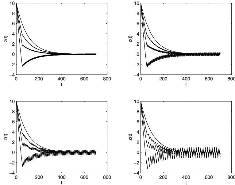
FIGURE 6. State trajectory for the system of Figure 2 for different values of \epsilon : (top left) \epsilon = 0 and g_3 as in (2.3); (top right) \epsilon = 0.8 ; (bottom left) \epsilon = 2 ; (bottom right) \epsilon = 5 . Chattering around the hyperplane \mathcal{H} increases with \epsilon .
