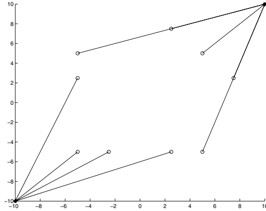
FIGURE 4. State trajectory in the phase plane from different initial states (circles) for g_3 as in (2.3) and C_2 < 0 . In evidence the two equilibria \pm \frac{D\bar{\omega}}{k} = \pm [10 \ 10]' (star).
