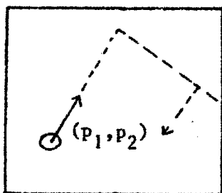
Weyl billiard
