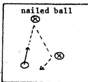
Sinai billiard
