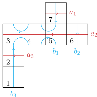
FIG. 1. — A square-tiled surface in the hyperelliptic locus of \Omega\mathcal{M}_3(2, 2)^{\text{odd}}
