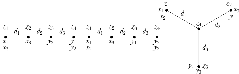
FIG. 3. — Possible stable limits of T
