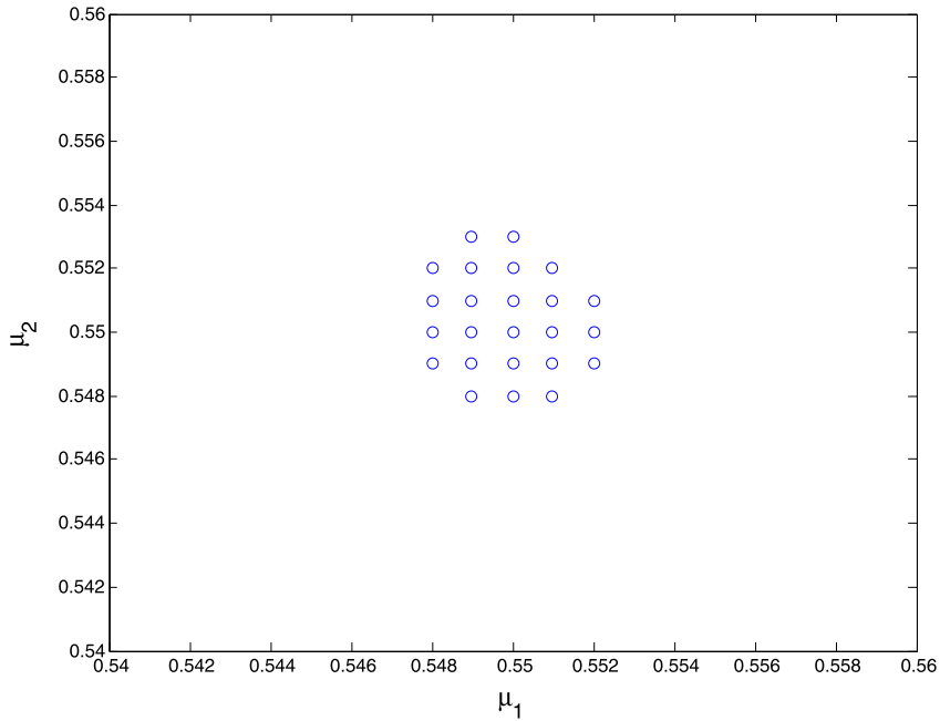
Fig. 1. The plot depicts the consistent set \mathcal{Y}_{\text{con}} in (6) for a particular realization. All the consistent parameter vectors are within the range \mu^* \pm \Delta\mu^* , with \mu^* = (0.55, 0.55) and \Delta\mu^* = (0.003, 0.003) ; note the restricted range of the axes relative to the full parameter domain \mathcal{D} = [0.4, 0.6]^2 .
