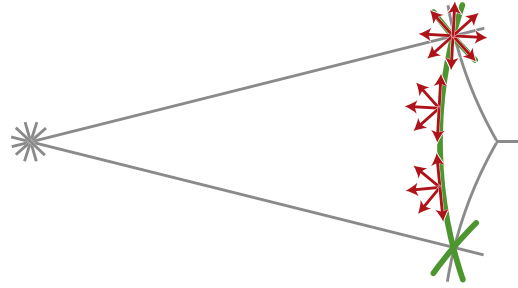
Fig. 1. The genus-one Birkhoff section for the geodesic flow on T^1\mathbb{H}^2/G_{2,3,t+4} constructed in [3] (here with t + 4 = 12 ). A fundamental domain for \mathbb{H}^2/G_{2,3,t+4} is obtained by gluing two symmetric hyperbolic right-angled triangles along their longest side. The geodesic that connects the two right angles induces a closed geodesic \gamma in \mathbb{H}^2/G_{2,3,t+4} . The Birkhoff section is made of those unit tangents to \gamma that point into one given side of \gamma (here the side of the order 12 vertex), plus the whole fiber of the order-2 point.
