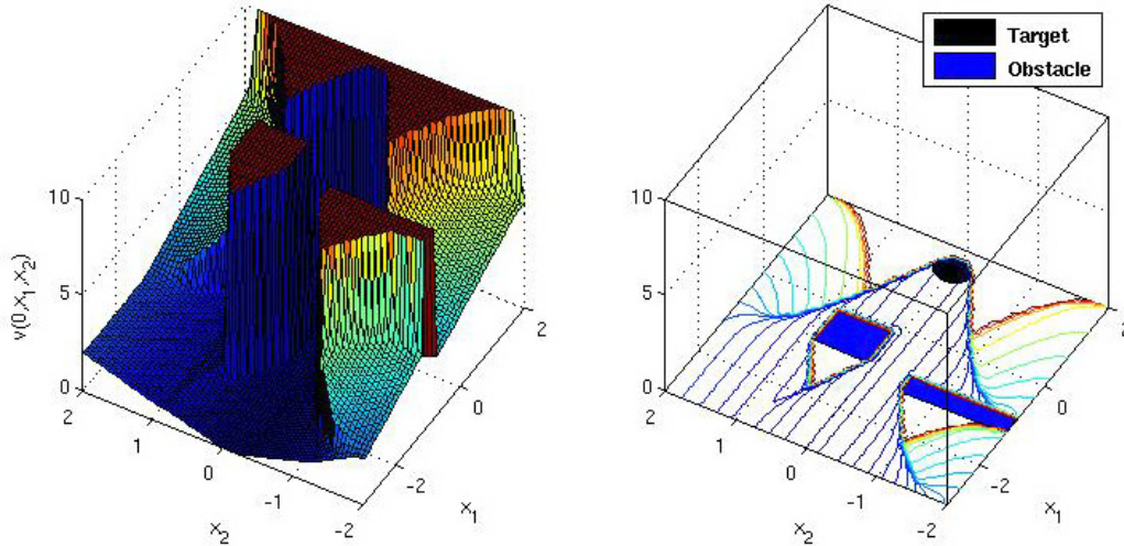
FIGURE 1. Left: values of v(t, \cdot) at time t = 0 . Right: iso-values in logarithmic scale. Here the values such that \vartheta(0, x_1, x_2) = 10 correspond to a non-reachable zone.
