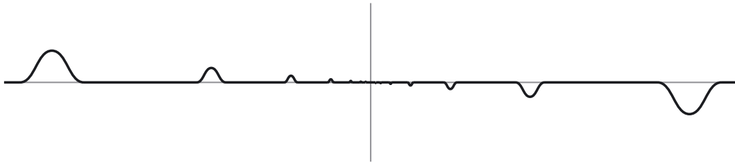
FIGURE 4. The graph of \xi .
