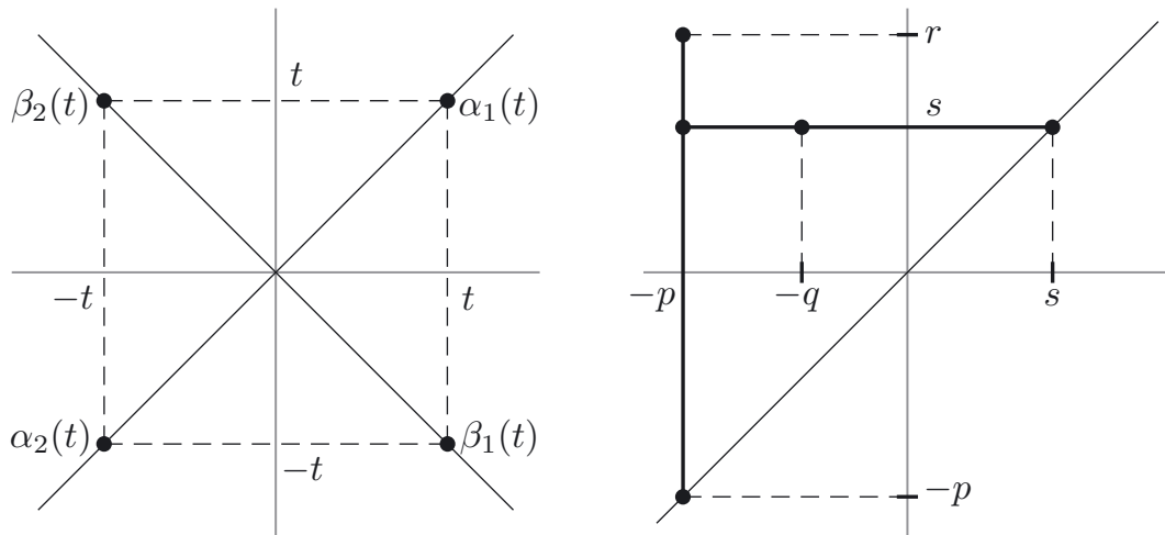
FIGURE 2. (a) Values of the functions \alpha_i, \beta_i, i = 1, 2 . (b) An illustration concerning of inequalities in (4.1) and (4.2).
