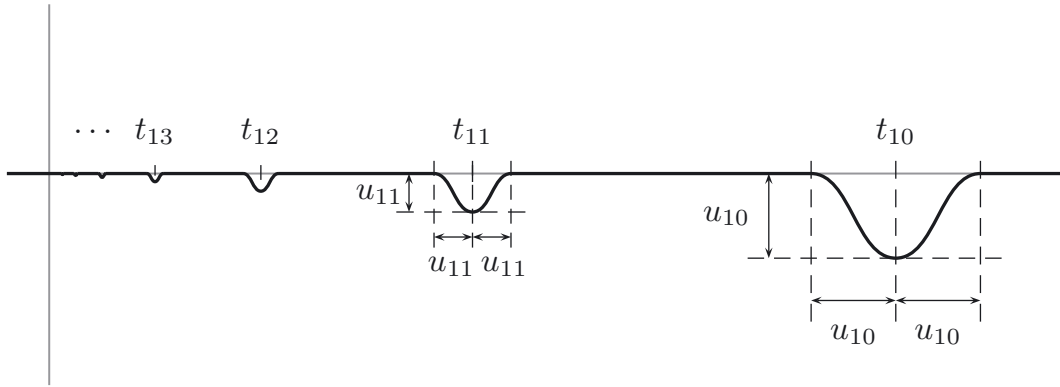
FIGURE 3. The graph of \psi .
