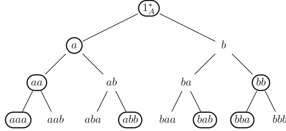
FIGURE 1. The tree representation of L_1 .
