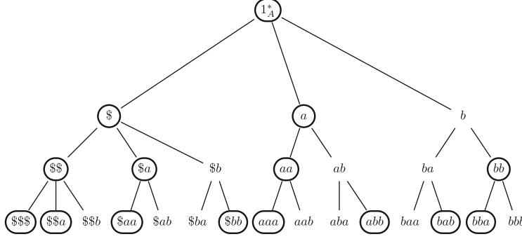
FIGURE 8. Tree representing K_1 .
