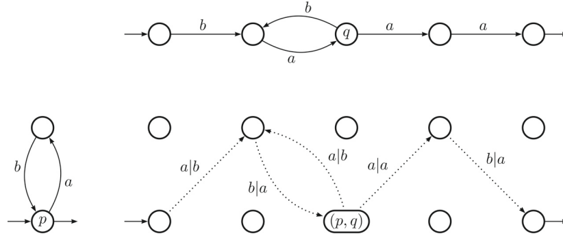
FIGURE 4. The synchronous product of \mathcal{A}_2 and \mathcal{B}_2 .
