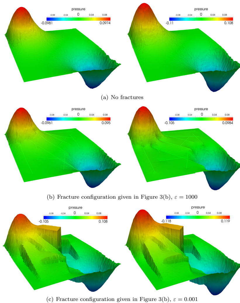
FIGURE 6. Example 3. Mimetic finite difference ( left ) and finite volume ( right ) computed pressures for different geometrical configurations and different choices of \varepsilon .
