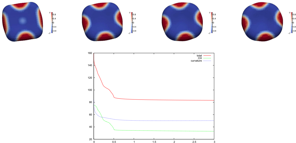
FIGURE 17. ( \alpha_{\pm} = 1, \bar{\alpha}_{\pm} = 0, \alpha_{-}^G = 0, \alpha_{+}^G = 0.5, \beta = 1 ) Plots of \mathfrak{C}^m on \Gamma^m at times t = 0.5, 1, 2, 3 . Below a superimposed plot of the total discrete energy \mathcal{E}_{\text{total}}^h , the discrete Cahn–Hilliard energy, and the discrete curvature energy over [0, 3] .
