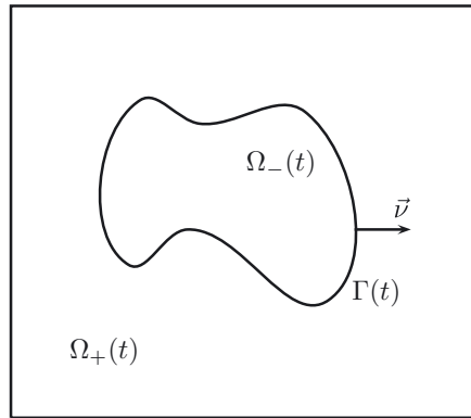
FIGURE 1. The domain \Omega in the case d = 2 .
