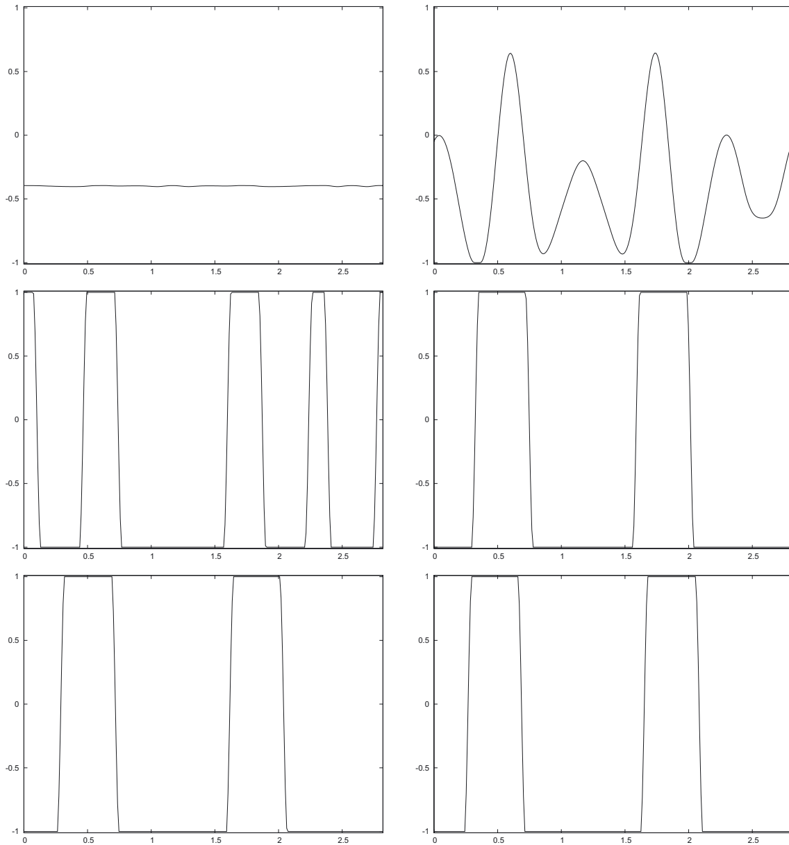
FIGURE 3. ( \alpha_{\pm} = 1 , \bar{\alpha}_- = -\frac{1}{2} , \bar{\alpha}_+ = -2 , \beta = 1 ) Flow for a smooth letter “U”. We show arclength plots of \mathfrak{C}^m at times t = 0, 0.001, 0.01, 0.1, 0.2, 1 .
