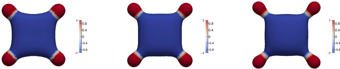
FIGURE 12. ( \alpha_{\pm} = 1, \bar{\alpha}_- = -\frac{1}{2}, \bar{\alpha}_+ = -2, \beta = 5 ) Plots of \mathfrak{C}^m on \Gamma^m at times t = 0.5, 1, 5 .
