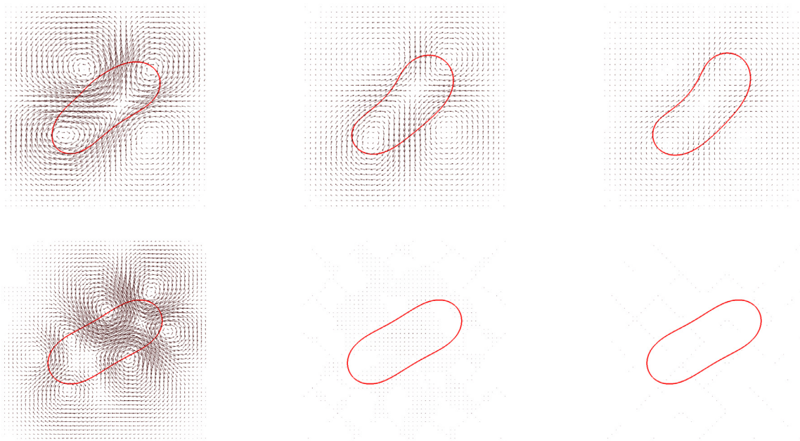
FIGURE 7. ( \alpha_{\pm} = 1 , \bar{\alpha}_{-} = 0.5 , \bar{\alpha}_{+} = 2 , \beta = 10 ) Visualization of the flow field \vec{U}^m at times t = 1, 2, 3 for the computation in Figure 6 (top), compared to the same computation with \mathfrak{C}^m = 1 constant throughout (bottom).
