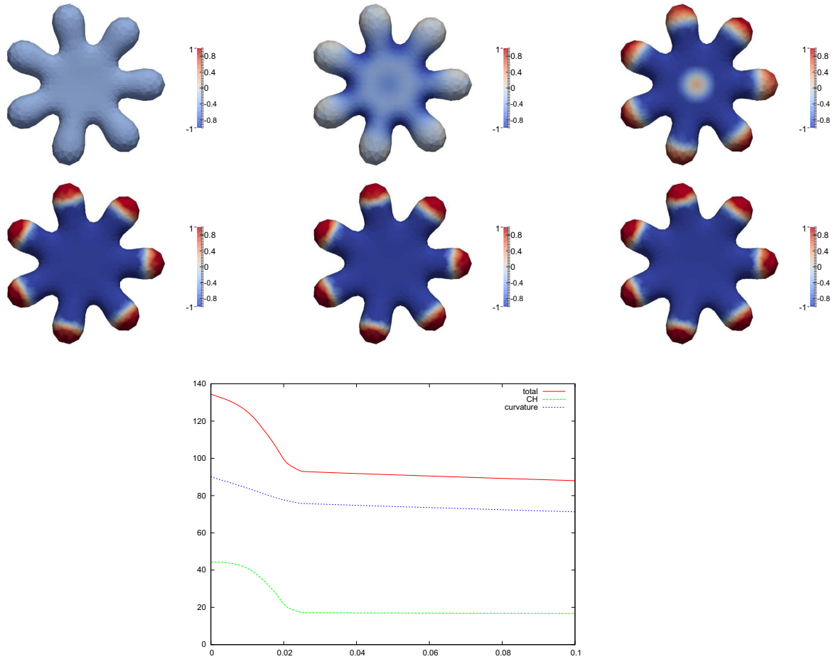
FIGURE 15. ( \alpha_{\pm} = 1 , \bar{\kappa}_{-} = -0.5 , \bar{\kappa}_{+} = -2 , \beta = 1 ) Spinodal decomposition on a seven-arm membrane. Plots of \mathfrak{C}^m on \Gamma^m at times t = 0, 0.01, 0.02, 0.03, 0.05, 0.1 . Below a superimposed plot of the total discrete energy \mathcal{E}_{\text{total}}^h , the discrete Cahn–Hilliard energy, and the discrete curvature energy over [0, 0.1] .
