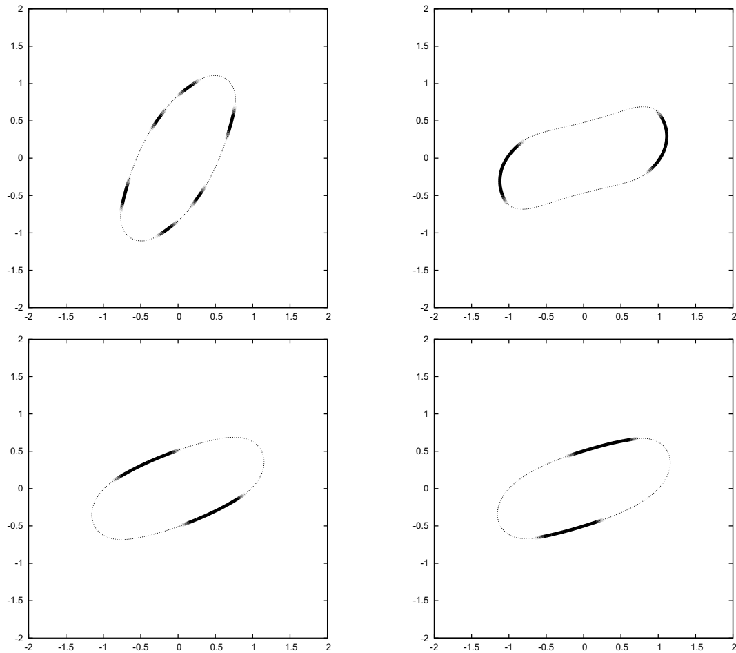
FIGURE 4. ( \alpha_- = 0.05 , \alpha_+ = 0.2 , \bar{\kappa}_\pm = 0 , \beta = 1 ) Shear flow with parameters as in (7.3a), leading to tank treading. The plots show the interface \Gamma^m , together with the concentration \mathfrak{C}^m at times t = 1, 11, 13, 15 (top left to bottom right).
