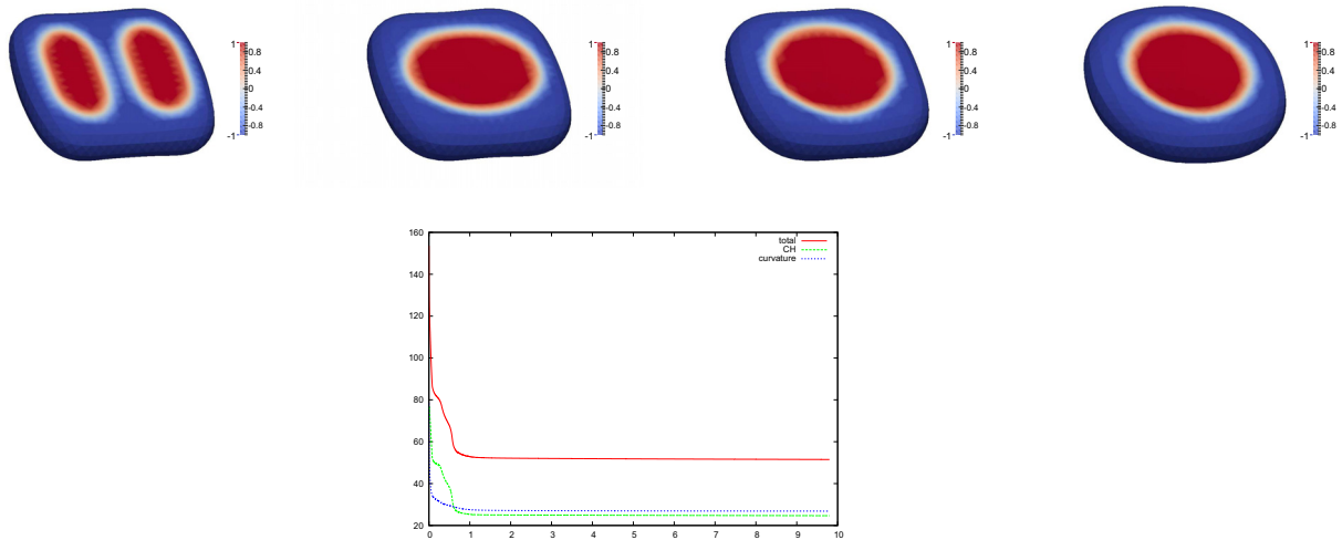
FIGURE 10. ( \alpha_- = \frac{1}{2}, \alpha_+ = 2, \bar{\alpha}_{\pm} = 0, \beta = 1 ) Plots of \mathfrak{C}^m on \Gamma^m at times t = 0.5, 1, 2, 10 . Compared to Figure 9, the final plot is less concave. Below a superimposed plot of the total discrete energy \mathcal{E}_{total}^h , the discrete Cahn–Hilliard energy, and the discrete curvature energy over [0, 10] .
