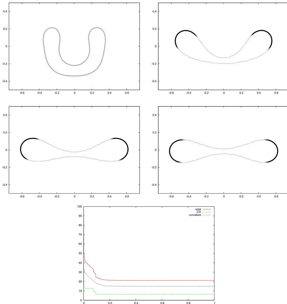
FIGURE 2. ( \alpha_{\pm} = 1 , \bar{\varkappa}_{-} = -\frac{1}{2} , \bar{\varkappa}_{+} = -2 , \beta = 1 ) Flow for a smooth letter “U”. We show \mathfrak{C}^m on \Gamma^m at times t = 0, 0.1, 0.2, 1 . Below a superimposed plot of the total discrete energy \mathcal{E}_{\text{total}}^h , the discrete Cahn–Hilliard energy, and the discrete curvature energy over [0, 1] .
