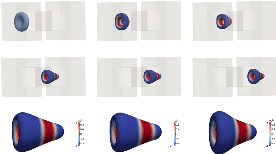
FIGURE 13. ( \alpha_- = 0.05, \alpha_+ = 0.1, \bar{\alpha}_{\pm} = 0, \beta = 1, \vartheta = 100 ) Flow through a constriction. Plots of \mathfrak{C}^m on \Gamma^m at times t = 0, 0.3, 0.5, 1, 1.2, 1.5 . Below we show enlarged plots of \mathfrak{C}^m on \Gamma^m at times t = 1, 1.2, 1.5 .
