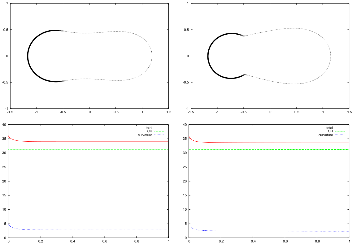
FIGURE 8. ( \alpha_{\pm} = 1 , \bar{\kappa}_{-} = -0.2 , \bar{\kappa}_{+} = -2 , \beta = 10 ) Solution at time t = 1 for the C^1 -case (left) and the C^0 -case (right). Below a superimposed plot of the total discrete energy \mathcal{E}_{\text{total}}^h , the discrete Cahn-Hilliard energy, and the discrete curvature energy over [0, 1] .
