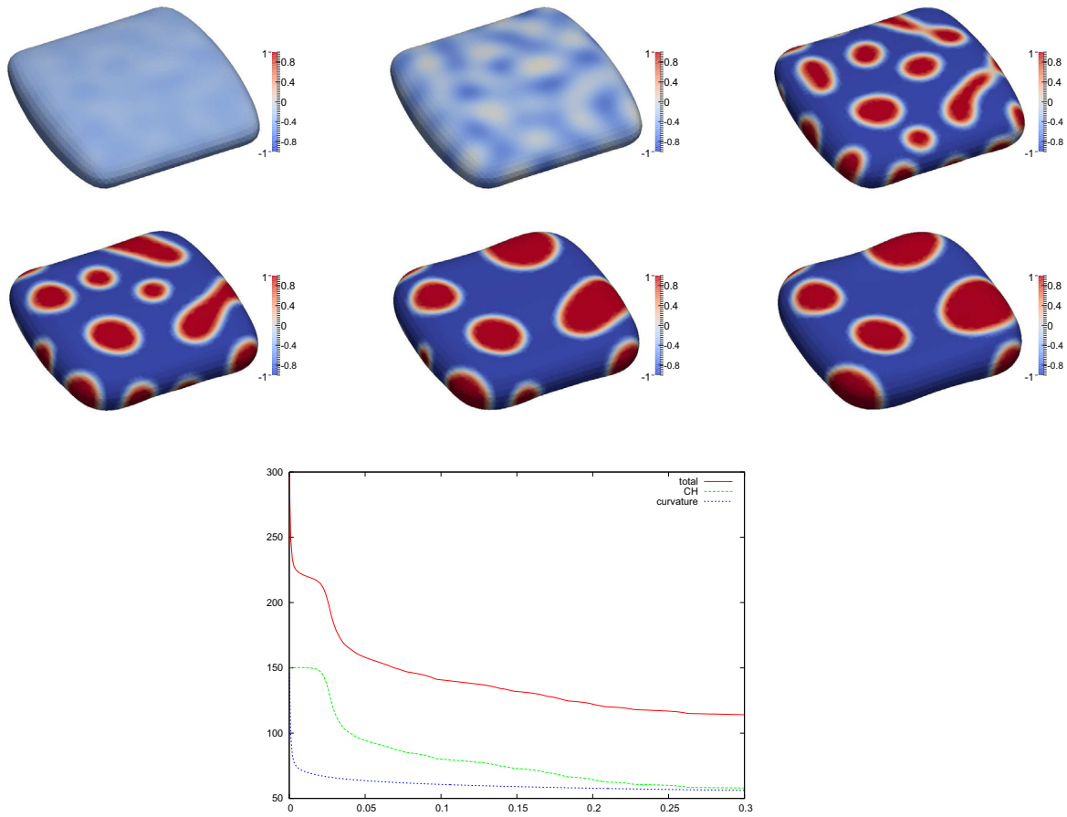
FIGURE 14. (\alpha_{\pm} = 1, \bar{\alpha}_{\pm} = 0, \beta = 1) Spinodal decomposition on a membrane. Plots of \mathfrak{C}^m on \Gamma^m at times t = 0.01, 0.02, 0.05, 0.1, 0.2, 0.3 . Below a superimposed plot of the total discrete energy \mathcal{E}_{\text{total}}^h , the discrete Cahn–Hilliard energy, and the discrete curvature energy over [0, 0.3] .
