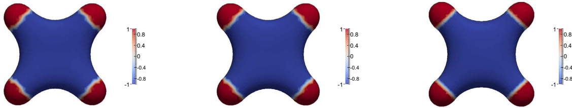
FIGURE 11. ( \alpha_{\pm} = 1, \bar{\alpha}_- = -\frac{1}{2}, \bar{\alpha}_+ = -2, \beta = 1 ) Plots of \mathfrak{C}^m on \Gamma^m at times t = 0.5, 1, 5 .
