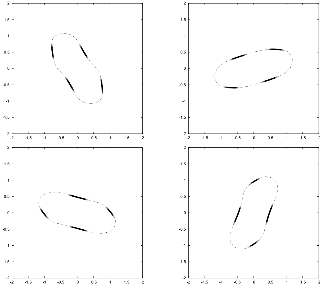
FIGURE 5. ( \alpha_- = 0.05 , \alpha_+ = 0.2 , \bar{\alpha}_\pm = 0 , \beta = 1 ) Shear flow with parameters as in (7.3b), leading to tumbling. The plots show the interface \Gamma^m , together with the concentration \mathfrak{C}^m at times t = 8, 11, 14, 17 (top left to bottom right).
