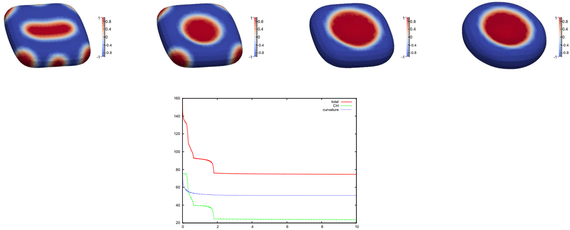
FIGURE 9. ( \alpha_{\pm} = 1, \bar{\alpha}_{\pm} = 0, \beta = 1 ) Plots of \mathfrak{C}^m on \Gamma^m at times t = 0.5, 1, 2, 10 . Below a superimposed plot of the total discrete energy \mathcal{E}_{total}^h , the discrete Cahn–Hilliard energy, and the discrete curvature energy over [0, 10] .
