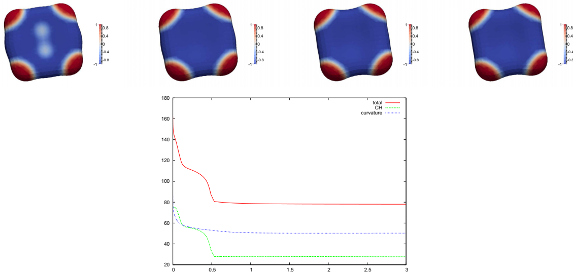
FIGURE 16. ( \alpha_{\pm} = 1, \bar{\alpha}_{\pm} = 0, \alpha_{-}^G = 0.5, \alpha_{+}^G = 0, \beta = 1 ) Plots of \mathfrak{C}^m on \Gamma^m at times t = 0.5, 1, 2, 3 . Below a superimposed plot of the total discrete energy \mathcal{E}_{\text{total}}^h , the discrete Cahn–Hilliard energy, and the discrete curvature energy over [0, 3] .
