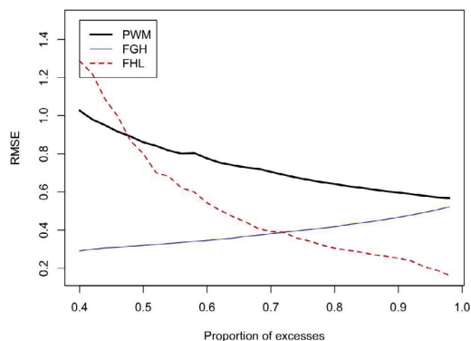
(b) RMSE for Burr(5, \frac{1}{2} ) model, n = 1000
