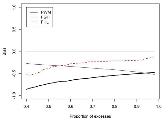
(a) Bias for Burr(5, \frac{1}{2} ) model, n = 1000
