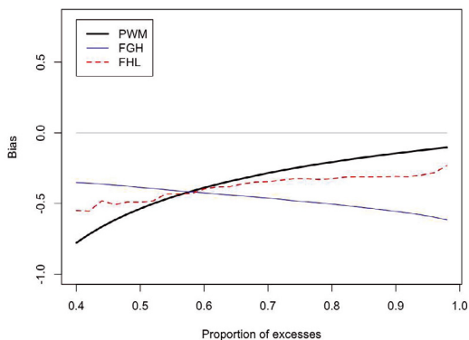
(c) Bias for Burr(10, \frac{1}{4} ) model, n = 1000
