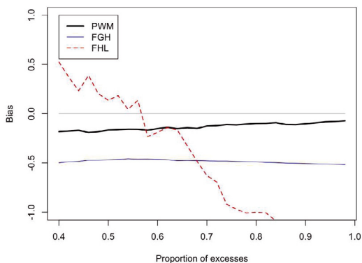
(e) Bias for model (4.1) with \gamma = 2/5 , n = 1000
