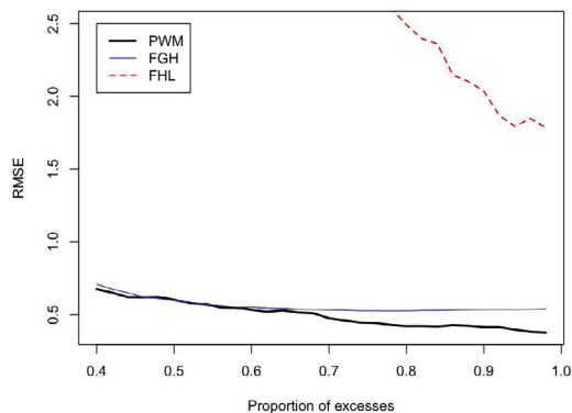
(f) RMSE for model (4.1) with \gamma = 2/5 , n = 1000
