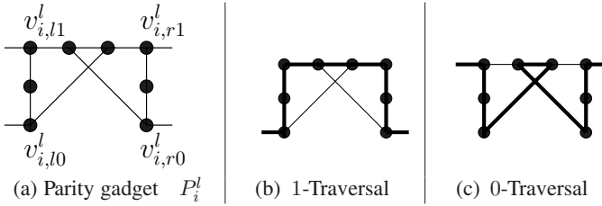
FIGURE 1. 0/1-Traversals of the parity gadget P_i^l . Traversed edges are displayed by thick lines.
