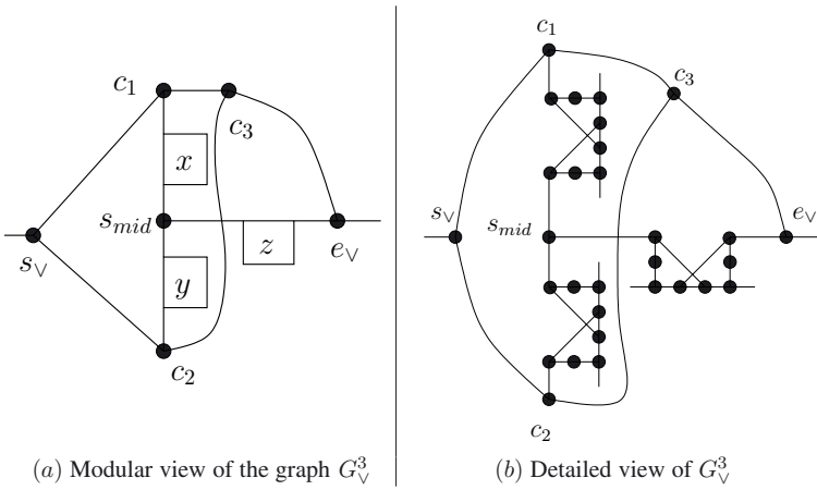
FIGURE 4. The graph G_V^3 corresponding to (x \vee y \vee z) .
