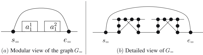
FIGURE 5. Graph G_=- corresponding to a_1^1 \oplus a_1^2 = 0 .
