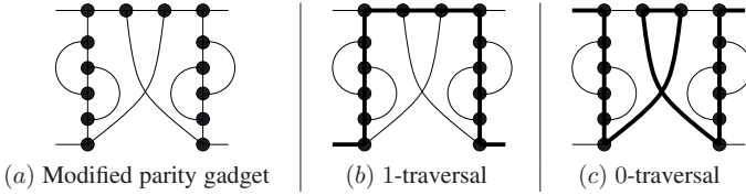
FIGURE 8. 0/1-Traversals of a modified parity gadget. The traversed edges are pictured by thick lines.
