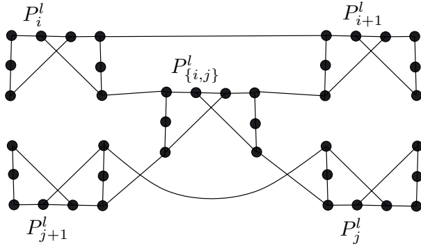
FIGURE 2. Construction simulating the equations x_i^l \oplus x_{i+1}^l = 0 , x_i^l \oplus x_{j+1}^l = 0 and x_j^l \oplus x_{j+1}^l = 0 .
