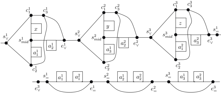
FIGURE 6. Modular view of the construction simulating x \oplus y \oplus z = 0 .
