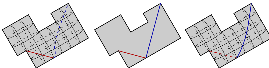
FIGURE 6. Flat spheres glued from two copies of a right-angled billiard. The angle by which the billiard table is rotated with respect to the horizontal position encodes the “phase” of the corresponding quadratic differential. A general generalized diagonal in the polygon gives rise to two distinct saddle connections on the flat sphere.
