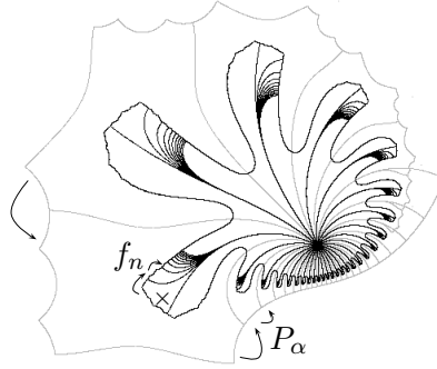
FIGURE 5. In the figure, \Omega^0 is the union of the sectors with gray boundaries. The domain \Omega^n is bounded by the black curve (amoeba) and some of the sectors in \Omega^n are shown. The map f_n corresponds to the n -th renormalization of P_\alpha . The critical point of P_\alpha is denoted by “ \times ” here.
