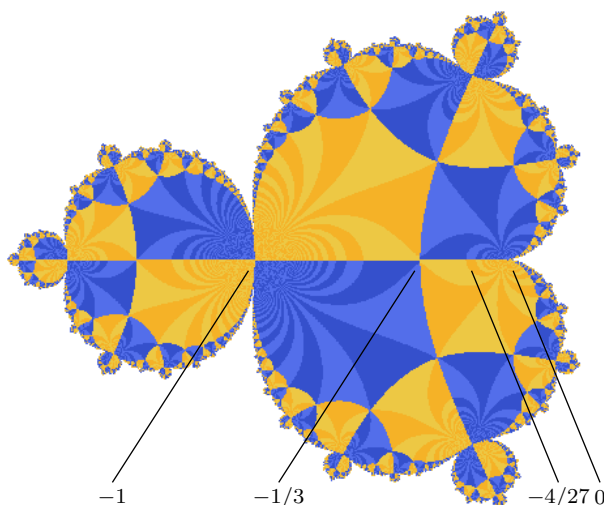
FIGURE 1. The dynamic plane of the polynomial P(z) = z(1+z)^2 , and the special points -1, -1/3, -4/27 , and 0 . The shades of blue are mapped by the Fatou coordinate to strips of width one in the upper half plane, while the shades of yellow are mapped by the Fatou coordinate to strips of width one in the lower half plane.
