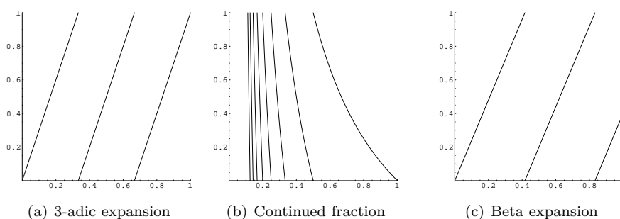
Figure 1: The graph of f^{-1} \bmod 1
