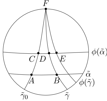
Figure 1. — Proof of Lemma 3.7
