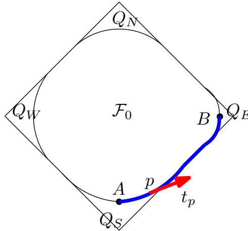
Figure 3.4. The curve \gamma (in blue) and the tangent vector t_p at a point p \in \gamma .
