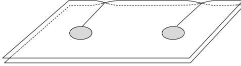
Figure 3.1. The domain of Z in the case q = 2
