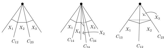
Figure 2.2. Examples: a R_3 -point, a S_4 -point and an E_3 -point.
