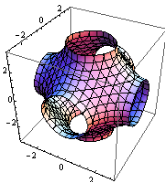
Figure 4.6. d = 3, \lambda = 1.45 .
