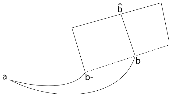
Figure 2.1. Solid line segments here (all except two) indicate geodesics in X , dotted line segments ( [b^-, b] and its translate to the right) indicate projected geodesics.
