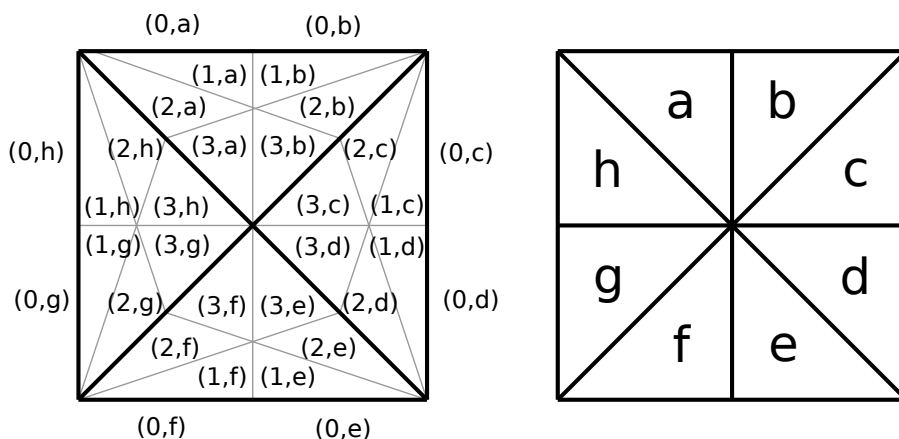
FIGURE 2. The flags of the pyramid over a square (left) and its base square (right).
