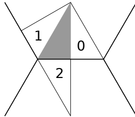
FIGURE 1. The action of the connections r_0 , r_1 and r_2 .
