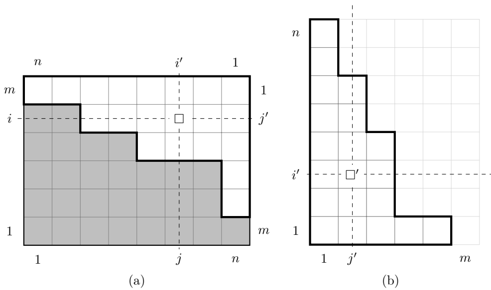
Figure 3. The relationship between contents within \lambda , \bar{\lambda}' and the rectangle n^m . (a) In this example m = 6 , n = 8 , \lambda = (8, 7, 7, 4, 2) is drawn with gray background. (b) The partition \bar{\lambda}' = (5, 3, 3, 3, 2, 2, 1, 1) is drawn with white background. Figure (a) shows how \lambda and \bar{\lambda}' are combined together within the rectangle n^m and how their respective coordinate systems are related. The content of \square' = (i', j') = (3, 2) \in \bar{\lambda}' is c(\square') = 2 - 3 = -1 , the same box in n^m is \square = (i, j) = (5, 6) with c(\square) = 1 and n + c(\square') = 7 = m + c(\square) .
