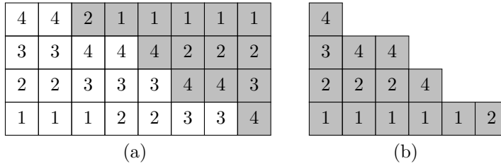
Figure 2. An example of the bijection from the proof of Claim 2.1 with m = 8 , n = 4 , and \nu = (7, 5, 4, 2) . (a) The original tableau is in white, and the (not rotated yet) complementary tableau of skew shape m^n/\nu is in gray. (b) The complementary tableau of shape \bar{\nu} = (6, 4, 3, 1) .
