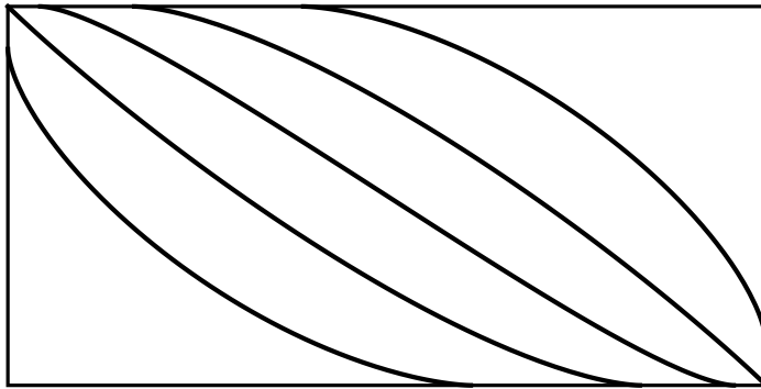
Figure 1. Asymptotic limit shapes of typical random Young diagrams which appear in Theorem 1.4, cf. [12, Figure 3]. We draw Young diagrams in the French convention. In this example the rectangle ratio is given by \frac{m}{n} = \frac{1}{2} . The limit curves correspond to \frac{p}{mn} \in \{\frac{1}{6}, \frac{2}{6}, \frac{3}{6}, \frac{4}{6}, \frac{5}{6}\} .
