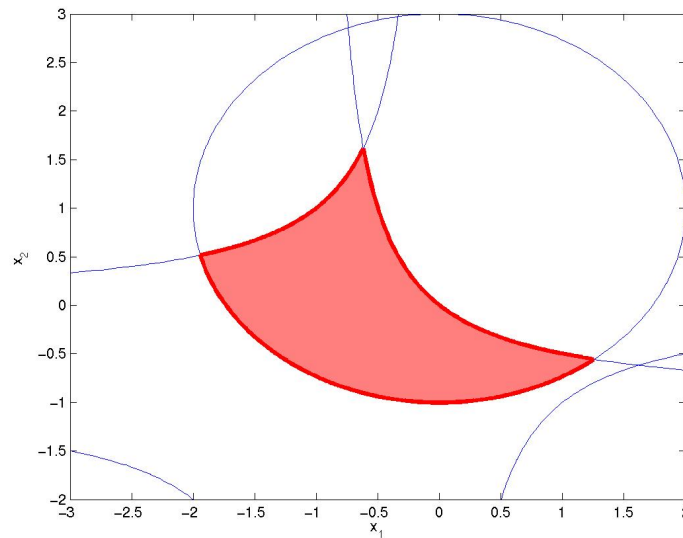
Figure 9.1: Nonconvex semialgebraic set X (in red).
