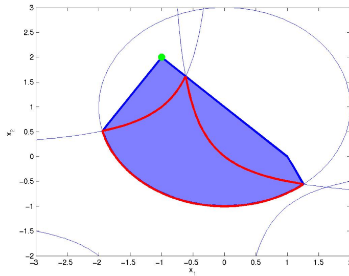
Figure 9.2: First spectrahedral shadow X_1 \supset X (in blue) with boundary of X (in red) and suboptimal point (in green).
