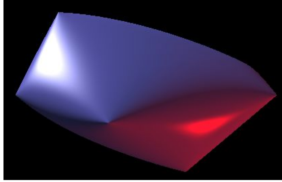
Figure 3.1: A spectrahedron.
