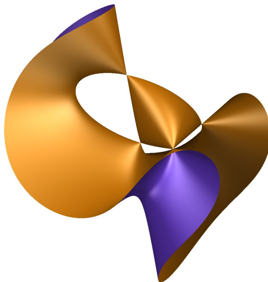
Figure 3.2: The Cayley cubic surface and its spectrahedron.
