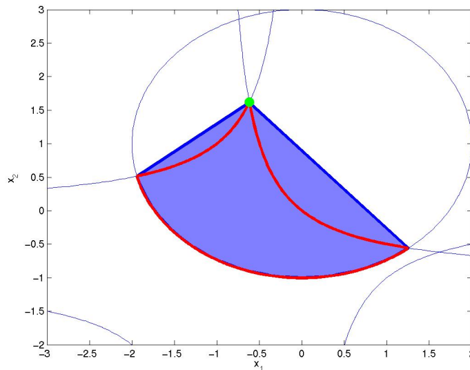
Figure 9.3: Second spectrahedral shadow X_2 \supset X (in blue) with boundary of X (in red) and optimal point (in green).
