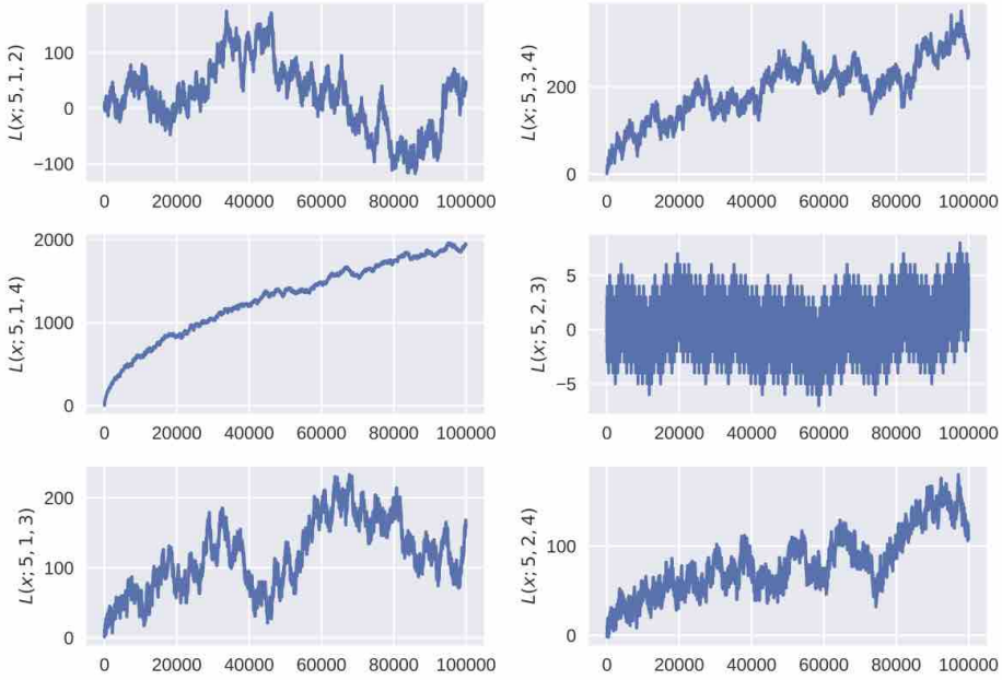
FIGURE 1.2. Combinations of L(x; 5, \cdot, \cdot) .
