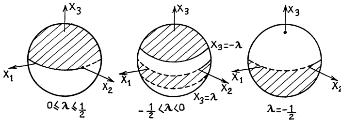
Fig. 1. — 0, 1-function \omega_{\psi, \lambda}(a) , a \in S with \psi = \begin{pmatrix} 1 \\ 0 \end{pmatrix} . Shadowed regions are mapped on 1.
