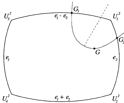
FIGURE 3. There is a curve of rank-one connections through any G \in \mathcal{D} that intersects two of the parabolic curves that bound \mathcal{D} .
