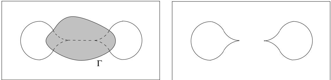
Figure 4: Left : disocclusion as a set of contours, E(D) < \infty Right : the associated solution u , E(u) = +\infty if p > 1 .
