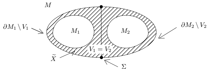
FIGURE 8. Gluing manifolds with corners
