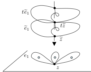
FIGURE 6. The complex R_n and its cover
