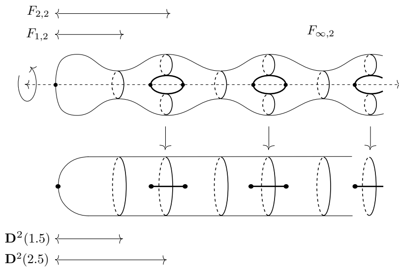
FIGURE 7. The surface F_{\infty,2} ramified over the plane
