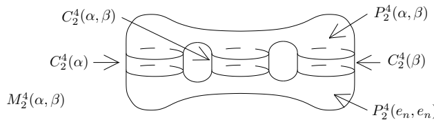
FIGURE 17. The manifold M_2^4(\alpha, \beta)
