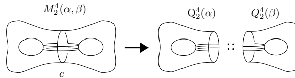
FIGURE 19. Splitting in two
