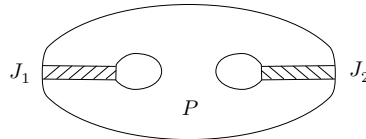
FIGURE 13. Cuts in the pair of pants
