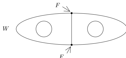
FIGURE 10. Splitting a pair of pants
