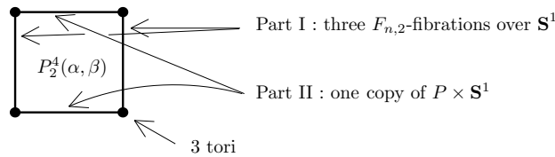
FIGURE 14. The manifold P_2^4(\alpha, \beta)
