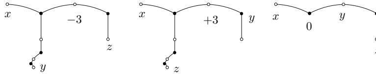
FIGURE 21. Orientation of a triangle in the tree
