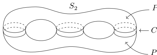
FIGURE 12. Surface of genus 2
