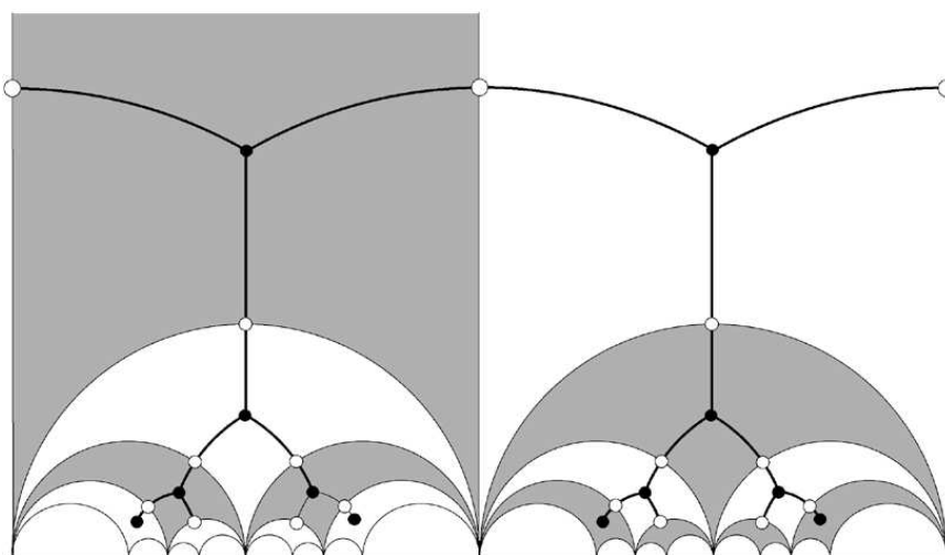
FIGURE 20. Action of \mathbf{SL}(2, \mathbf{Z}) on the tree
