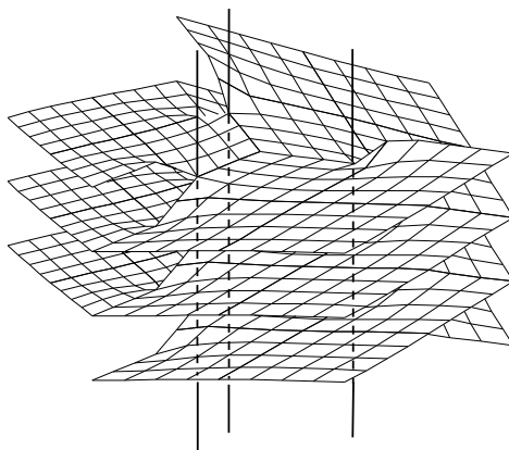
FIGURE 5. Covering of the punctured disc
