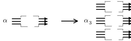
FIGURE 11. Juxtaposition of a braid
