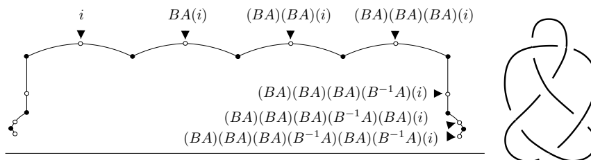
FIGURE 22. \Phi((BA)(BA)(BA)(B^{-1}A)(BA)(B^{-1}A)) = 2 and the knot \overline{6}_2
