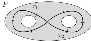
FIGURE 9. Pair of pants
