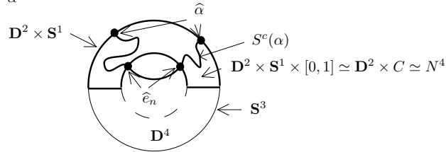
FIGURE 16. Pushing the Seifert surface in 4-ball
