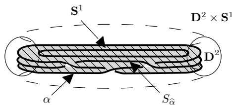
FIGURE 15. Seifert surface
