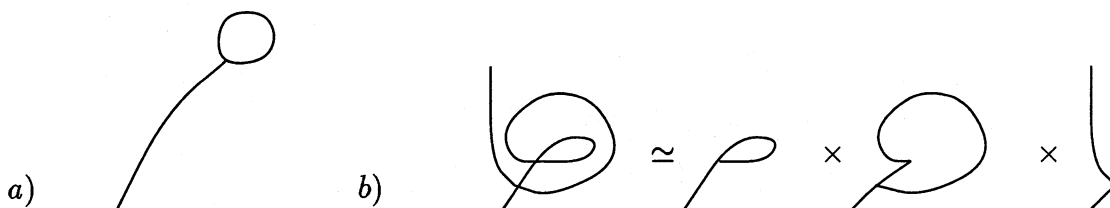
Figure 2.1: a) A lasso. b) An example of decomposition.
