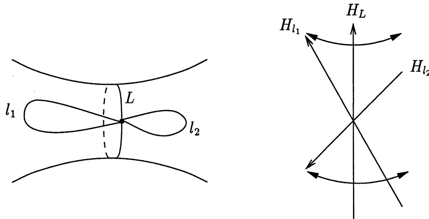
Figure 5.2: Lack of information about the joint class [H_L, H_{l_1}, H_{l_2}] when G = SO(3) .
