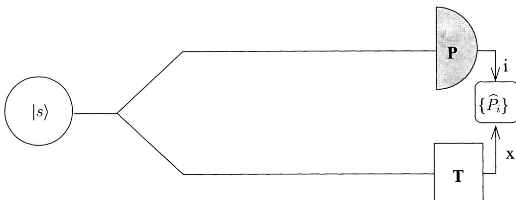
Figure 2.3: Experimental set-up to determine the POVM associated to an unknown photocounter \mathbf{P} . We use it to measure a known bipartite state |s\rangle , jointly with a tomographer \mathbf{T} . The photocounter gives a result i and the tomographer a result x . From these samples, we construct an estimator \{\hat{P}_i\} of the self-adjoint operators associated to the results \{i\} by the photocounter \mathbf{P} .
